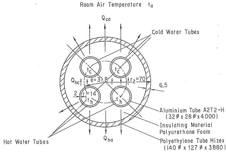
Fig. A-3. Heat flow in an insulated pipe unit to feed hot and cold water in low temperature room.
